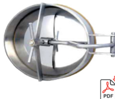
Cod. P2-A31 (PED) 520 x 420 mm +6,0 bar
