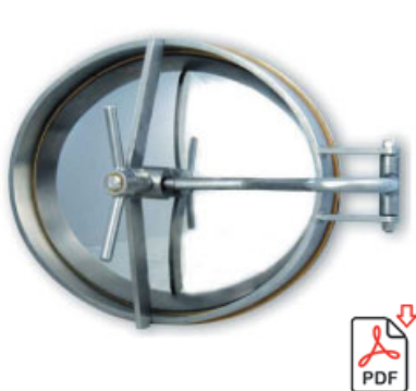
Cod. P2-A15 520 x 420 mm +8,0 bar
